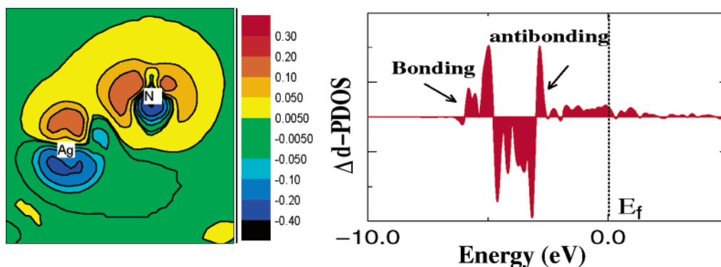
Figure 3. Bonding of N on Ag{111}. (a) Charge density difference contour plot (unit: e^{-}/\text{\AA}^3 ) cutting through the N–Ag bonding plane, constructed by subtracting the total charge densities of the adsorbed system from those of the separated N atom and clean Ag{111} surface. Positive values (red) represent an electron density increase. (b) The difference of the d-projected density of states (d-PDOS) of the Ag atom depicted in (a) before and after N adsorption.
